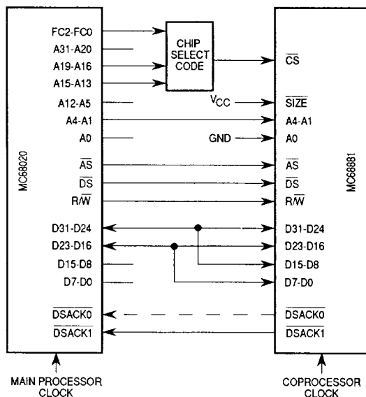
Figure 12. 16-Bit Data Bus Coprocessor Connection
