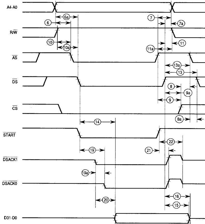
Figure 18. Asynchronous Read Cycle Timing Diagram
