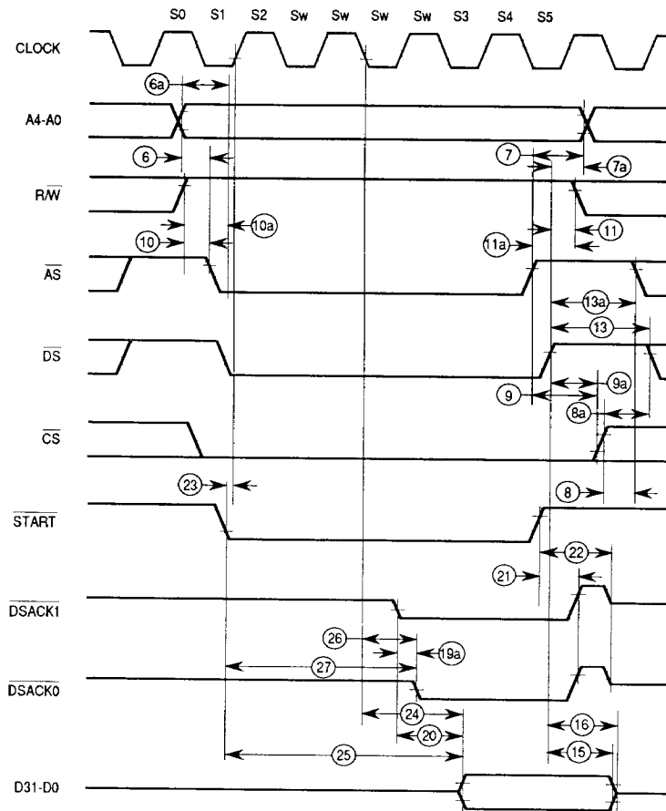
Figure 20. Synchronous Read Cycle Timing Diagram
