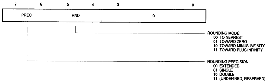
Figure 3. Mode Control Byte
