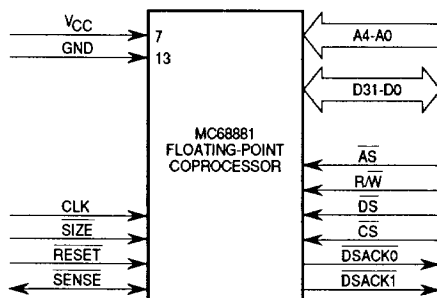
Figure 10. Functional Signal Groups
