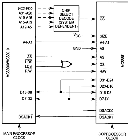
Figure 14. 16-Bit Data Bus Peripheral Processor Connection
