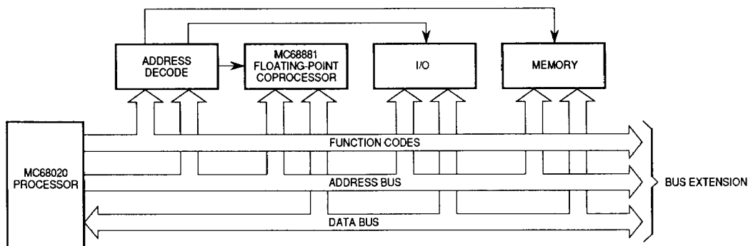
Figure 7. Typical Coprocessor Configuration
