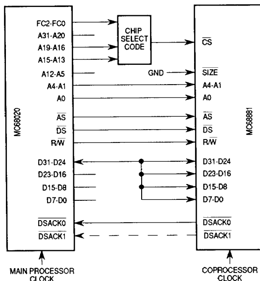
Figure 13. 8-Bit Data Bus Coprocessor Connection
