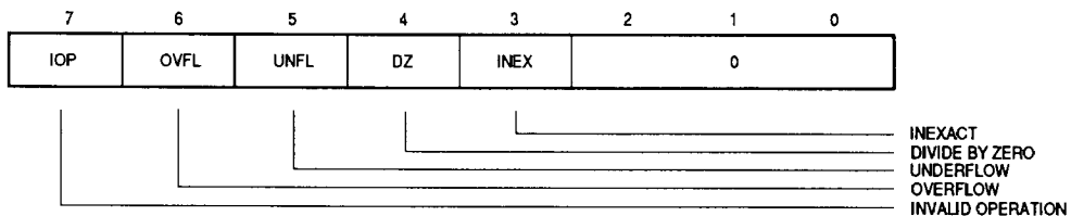
Figure 6. Accrued Exception Byte
