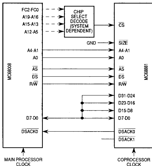
Figure 15. 8-Bit Data Bus Peripheral Processor Connection
