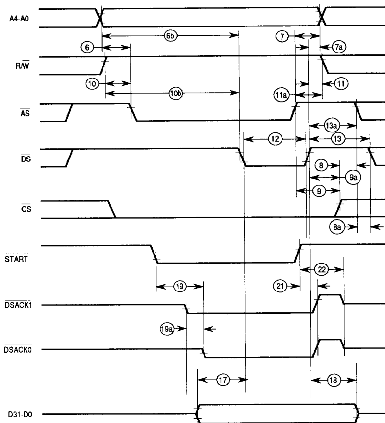
Figure 19. Asynchronous Write Cycle Timing Diagram
