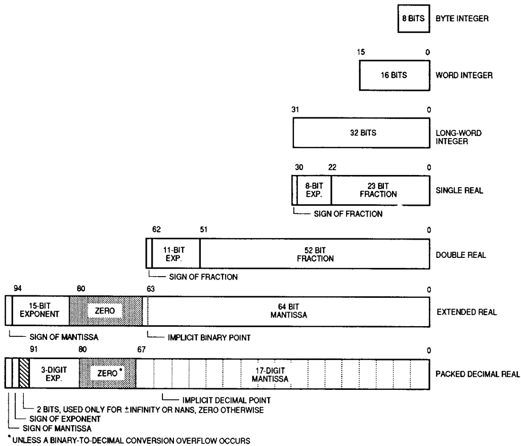
Figure 9. Data Format Summary
