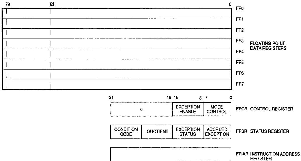
Figure 1. Programming Model
