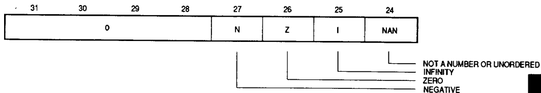
Figure 4. Condition Code Byte
