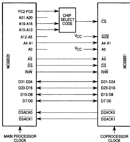
Figure 11. 32-Bit Data Bus Coprocessor Connection
