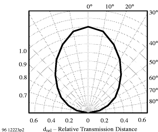
Figure 12. Directivity
