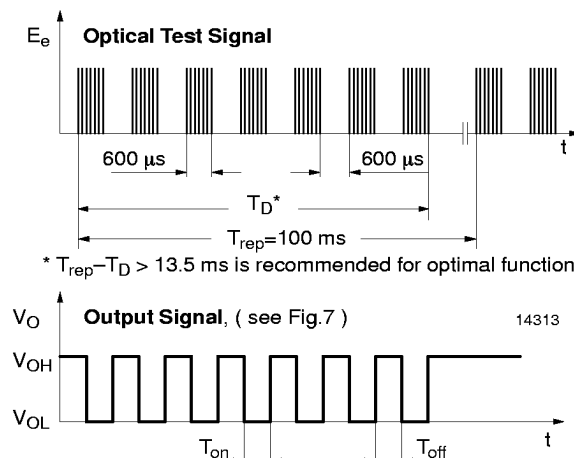
Figure 6. Output Function
