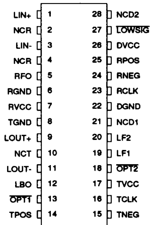
28-Pin DIP
