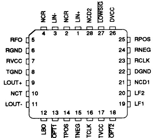
28-Pin PLCC
