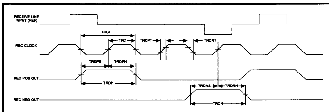
FIGURE 2: Receive Waveforms
