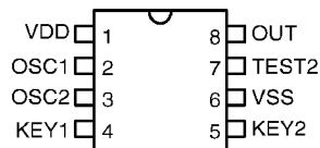
HT2823 – 8 DIP/SOP
