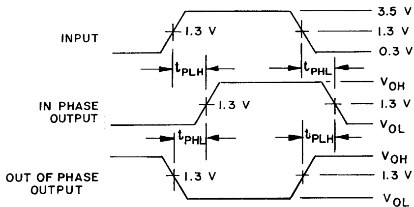
VOLTAGE WAVEFORMS PROPAGATION DELAY TIMES
