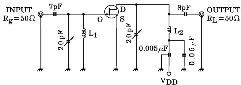
Fig.1 100MHz G_{ps} , NF TEST CIRCUIT
