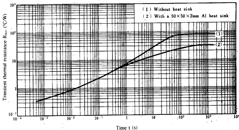
R_{th(t)} - t
