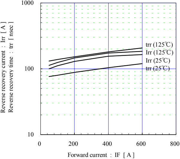
Reverse recovery characteristics (typ.) Vcc=300V, VGE=±15V, Rg=6.8Ω
