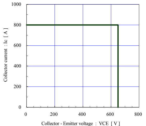
Reverse bias safe operating area (max.) +V_{GE}=15V , -V_{GE}\leq 15V , R_g\geq 6.8\Omega , T_j\leq 125^\circ C
