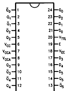
24-Pin DIP
