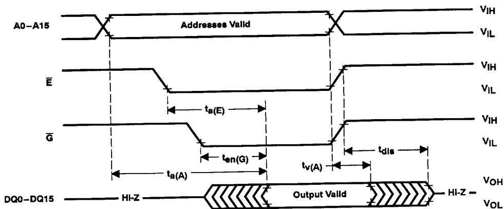
Figure 3. Read-Cycle Timing
