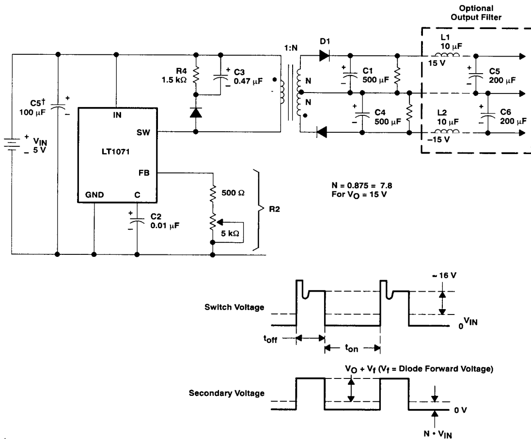
Figure 23. Totally Isolated Converter
