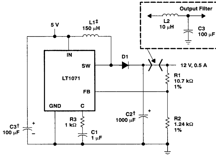
Figure 24. Boost Converter (5 V to 12 V)
