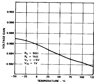
Figure 4. Gain vs. Temperature
