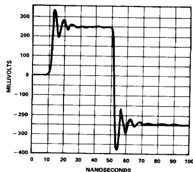
Figure 8. Small-Signal Settling ( \pm 250\text{mV} Square Wave Input)
