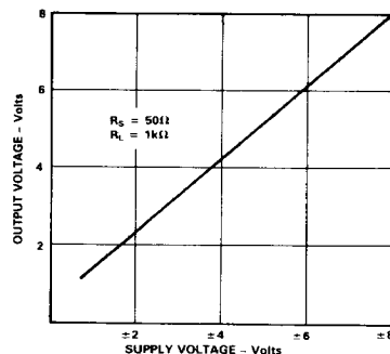
Figure 5. Output Voltage vs. Supply Voltage
