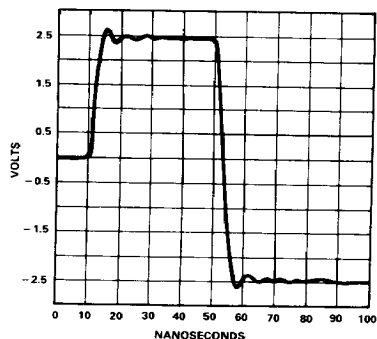
Figure 9. Large-Signal Settling ( \pm 2.5\text{V} Square Wave Input)
