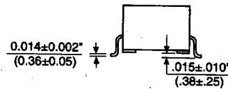
END VIEWS
