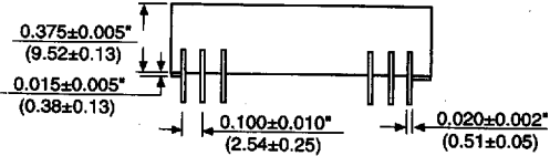
SIDE VIEWS
