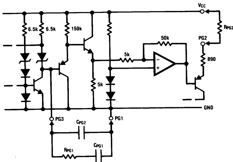
FIGURE 6. Pulse Gate Controls
