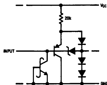
FIGURE 15. Logic Inputs
