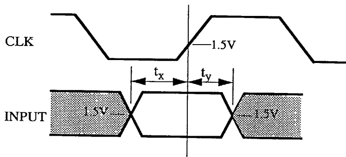
Figure 5.2. Setup and Hold Timings
