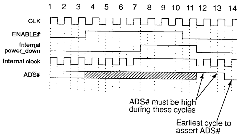
Figure 3.10. Power-down Timing
