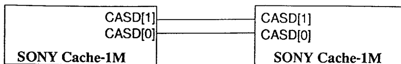
Figure 4.4. CASD signals
