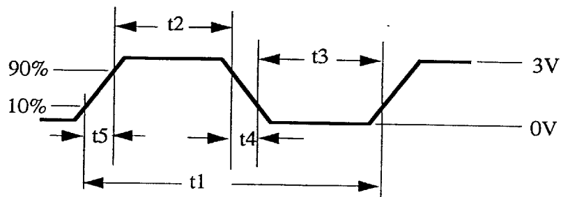
Figure 5.1. Clk Waveform
