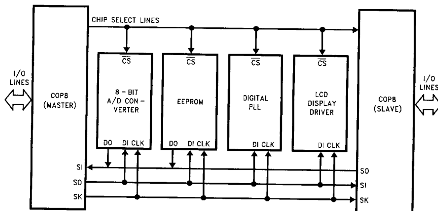
FIGURE 7. MICROWIRE/PLUS Application
