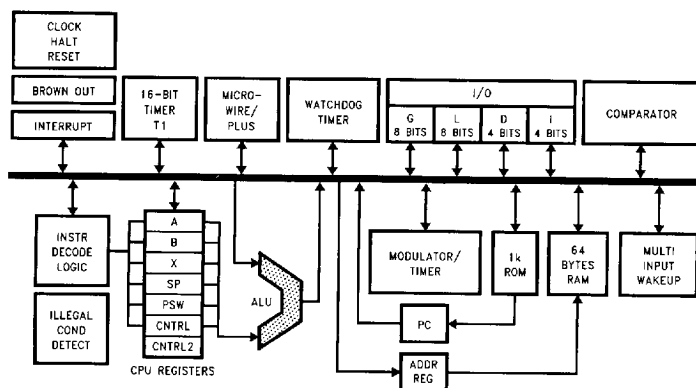
FIGURE 1. Block Diagram
