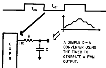
FIGURE 11. Timer Application
