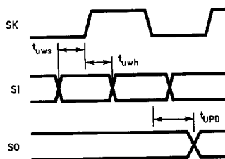
FIGURE 2. MICROWIRE/PLUS Timing
