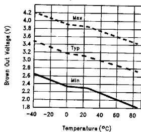
Brown Out Voltage vs Temperature
