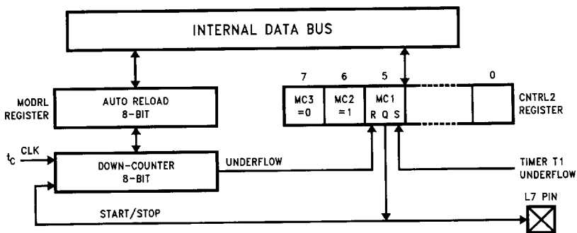
FIGURE 14. Mode 2a: 50% Duty Cycle Output
