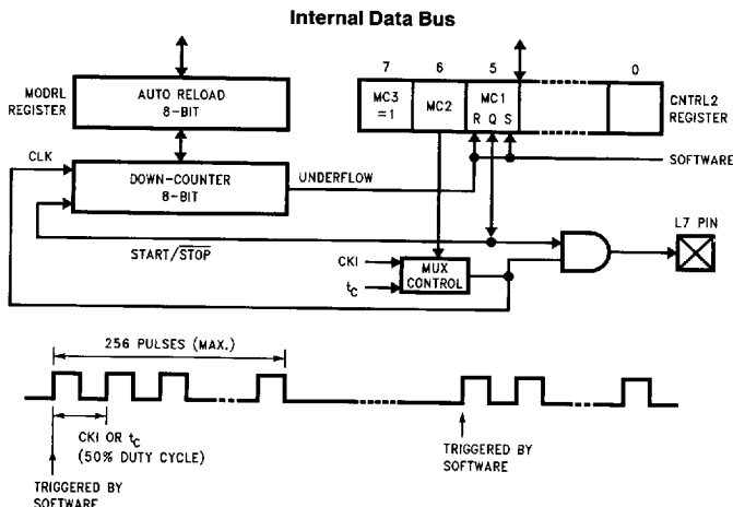
FIGURE 13. Mode 1: Modulator Block Diagram/Output Waveform
