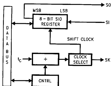
FIGURE 6. MICROWIRE/PLUS Block Diagram
