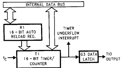
FIGURE 8. Timer/Counter Auto Reload Mode Block Diagram
