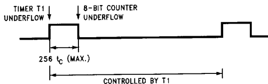
FIGURE 15. Mode 2b: Variable Duty Cycle Output
