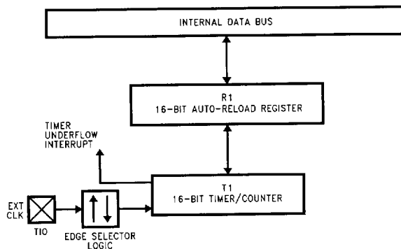
FIGURE 9. Timer in External Event Counter Mode
