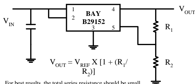
Fig. 2 Adjustable Output Voltage Regulator
