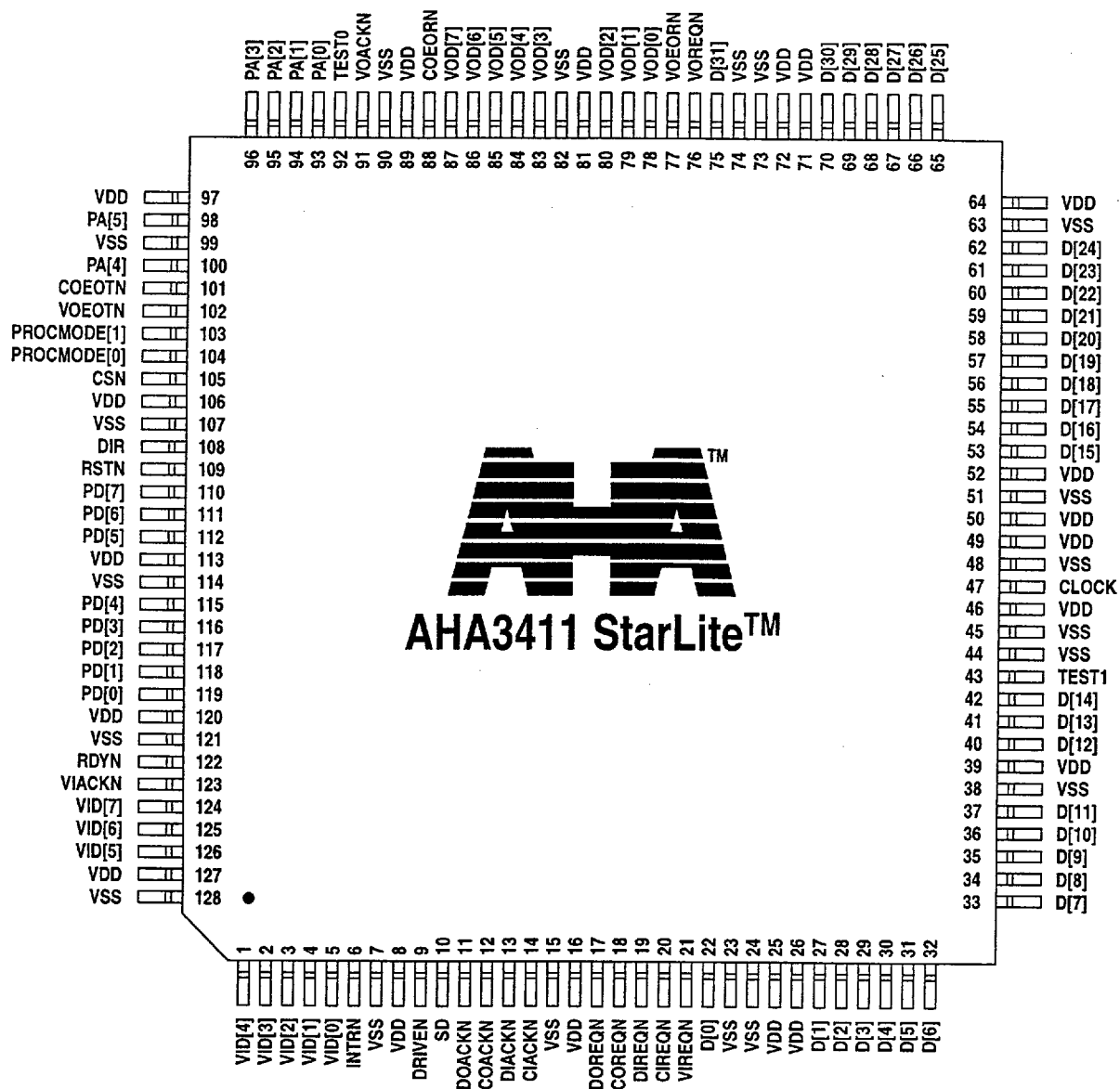
Figure 16: Pinout
