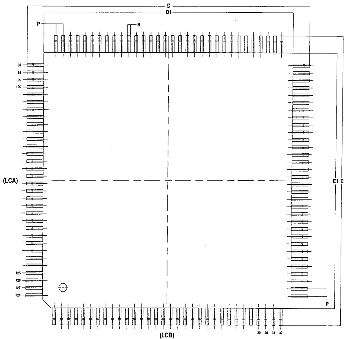
DETAIL A
