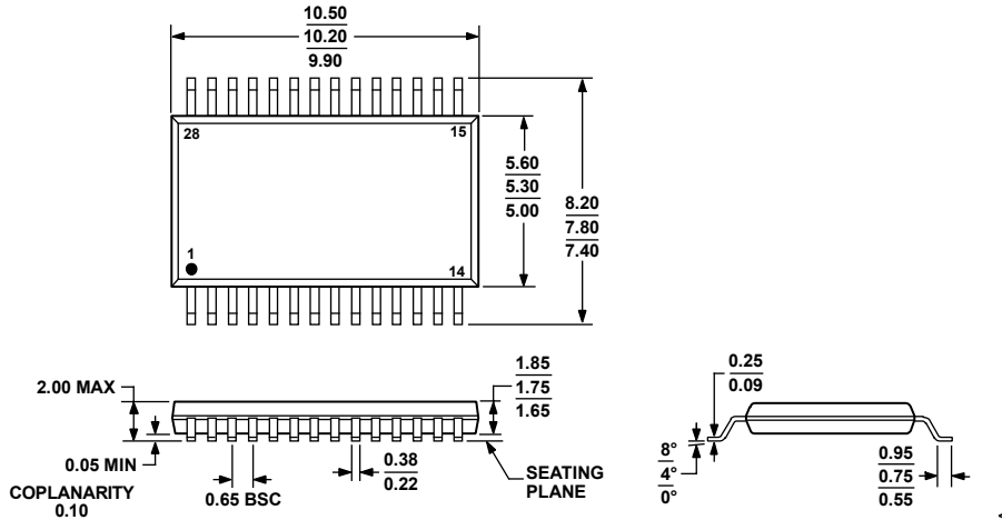
Figure 13. 28-Lead Shrink Small Outline Package [SSOP] (RS-28)
