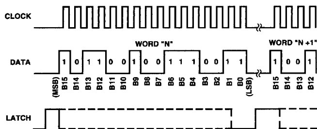
Figure 6. Write Cycle for 4–20 mA Operation
