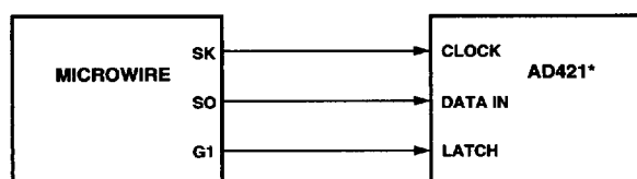
Figure 9. AD421 to MICROWIRE Interface
