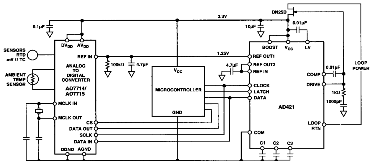
Figure 14. AD421 in Smart Transmitter Application
