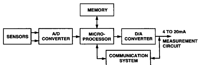
Figure 16. Smart and Intelligent Transmitter
