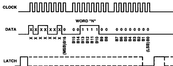
Figure 7. Write Cycle for Programming Alarm Current Data
