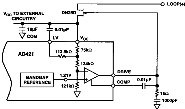
Figure 3. AD421 Voltage Regulator Circuit to Provide V_{CC} = 3.3 V
