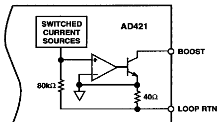
Figure 4. Current Amplifier
