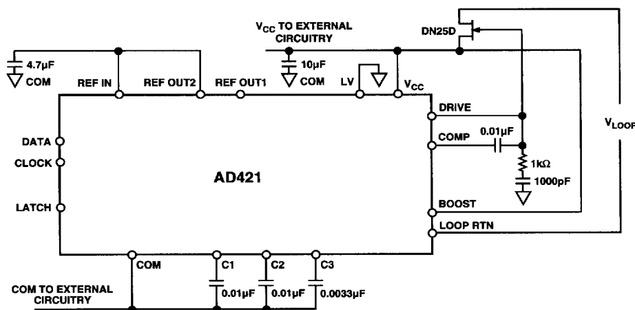
Figure 11. Basic Connection Diagram
