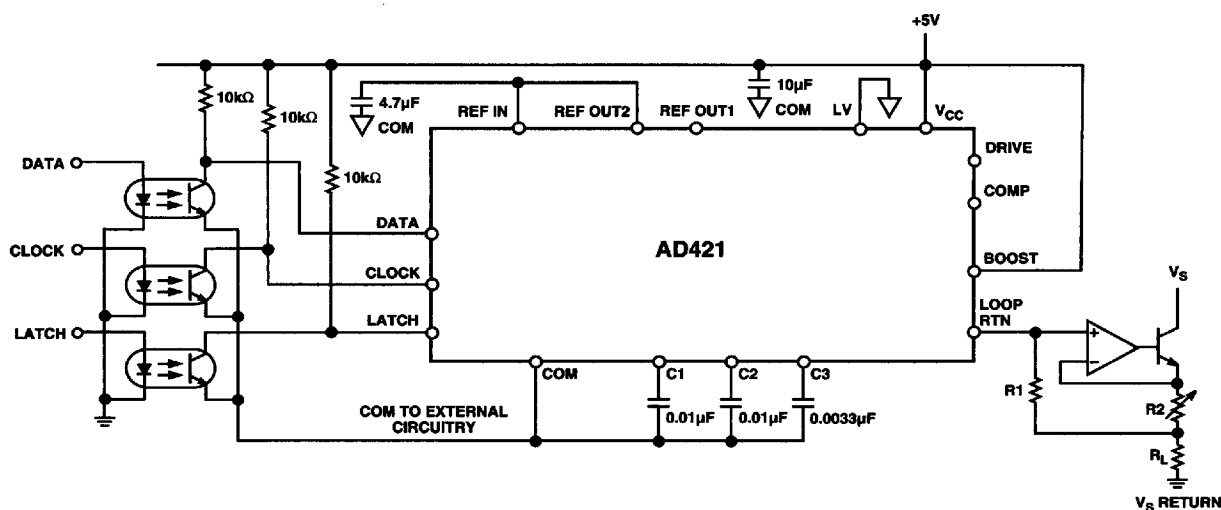
Figure 18. AD421 in Programmable Current Source/Sink
