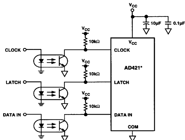
Figure 10. Opto-Isolated Interface
