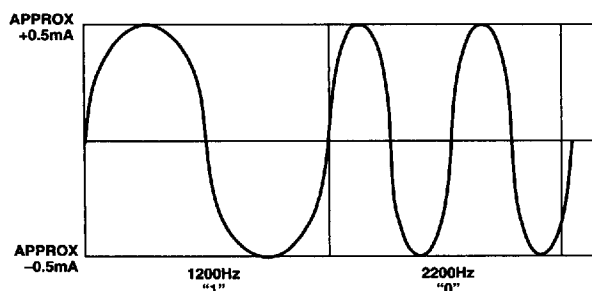
Figure 15. HART Transmission of Digital Signals
