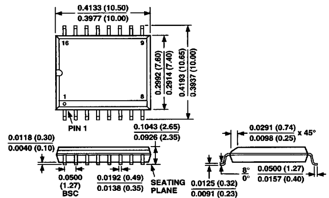
16-Lead (Wide Body) Small Outline Package (R-16)
