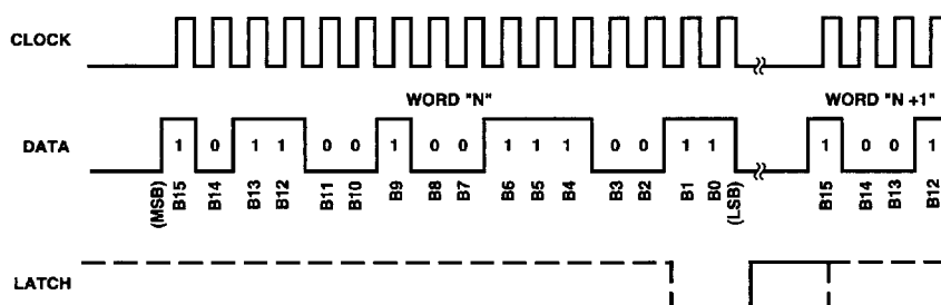
Figure 1. Serial Interface Waveforms (Normal Data Load)
