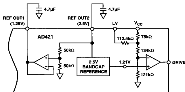
Figure 5. Reference Section
