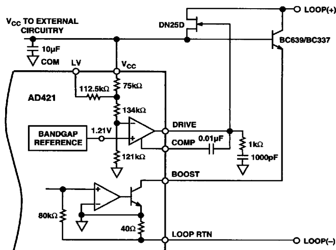
Figure 12. External NPN Transistor Reduces Power Load on FET
