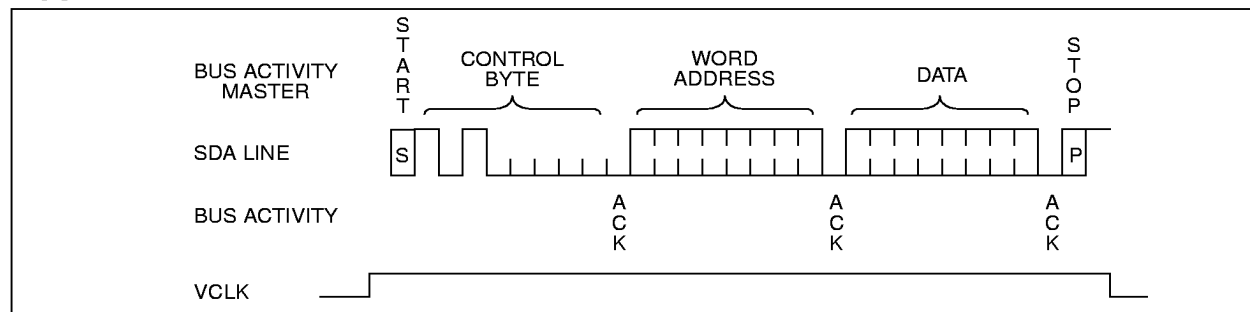
FIGURE 4-2: VCLK WRITE ENABLE TIMING
