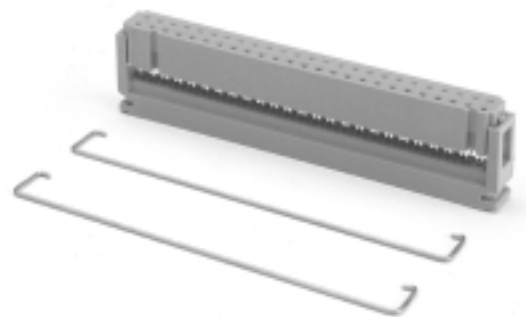
SOCKET CONNECTOR
