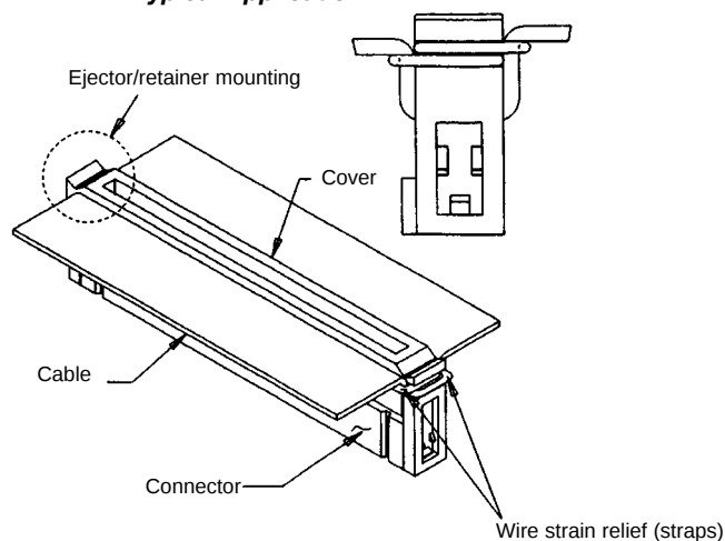
Typical Application
