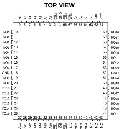
FIG. 3 PIN CONFIGURATION FOR WE128K32-XG2TX AND WE128K32-XG1UX
