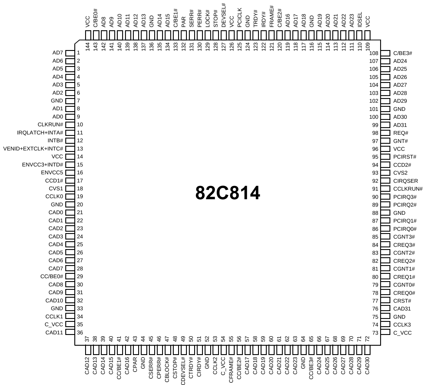
Figure 3-1 Pin Diagram
