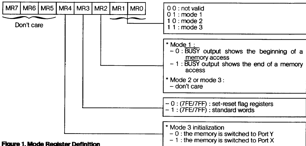
Figure 1. Mode Register Definition
