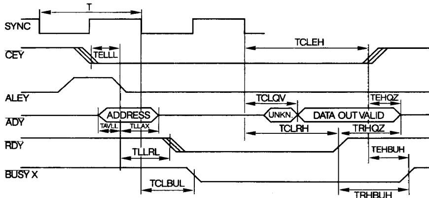
TIMING DIAGRAM WHEN A READ OPERATION IS COMPLETED FROM PORT X PRIOR TO PORT Y ACCESS
