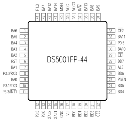
44-Pin MQFP
