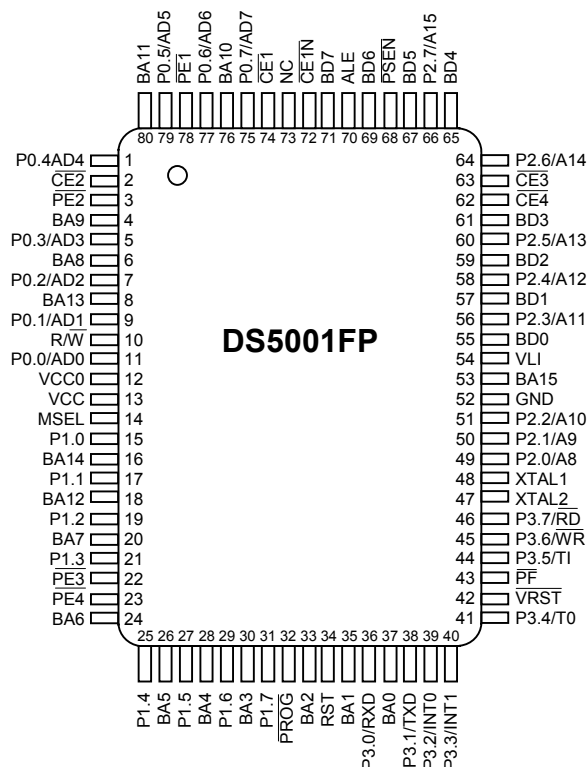
80-Pin MQFP
