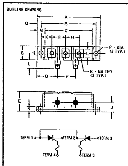
100-1400 Volts CDL3 — 40 Outline Drawing
