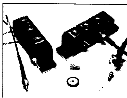
CDL3 — 40 Dual SCR Light-Triggered POW-R-BLOK™ Module 40 Amperes/100-1400 Volts
