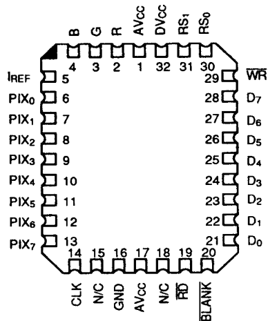
32-PIN PLCC
