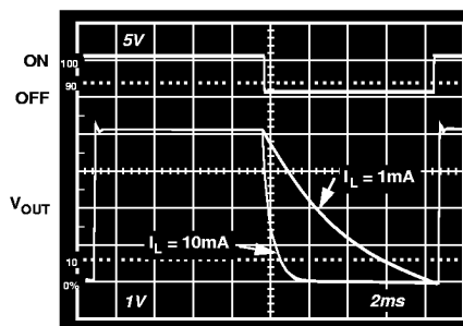
Figure 11a. Sleep Response Time
