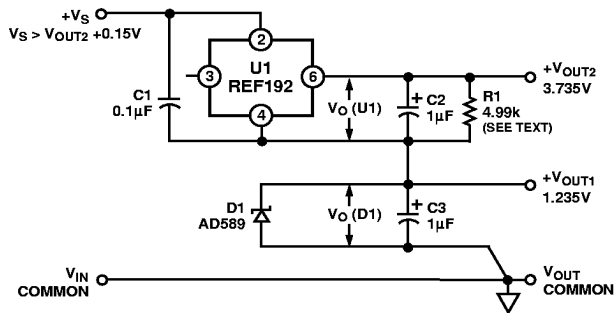
Figure 20. Stacking Voltage References with the REF19x
