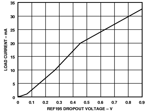
Figure 13. Dropout Voltage vs. Load Current
