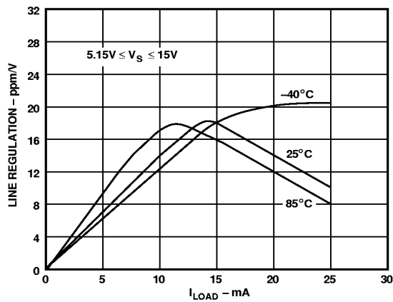
Figure 2. REF195 Line Regulation vs. I_{LOAD}
