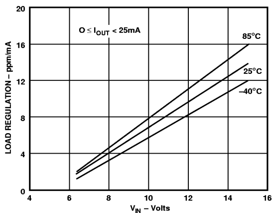
Figure 3. REF195 Load Regulation vs. V_{IN}
