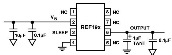
Figure 15. Basic Voltage Reference Configuration
