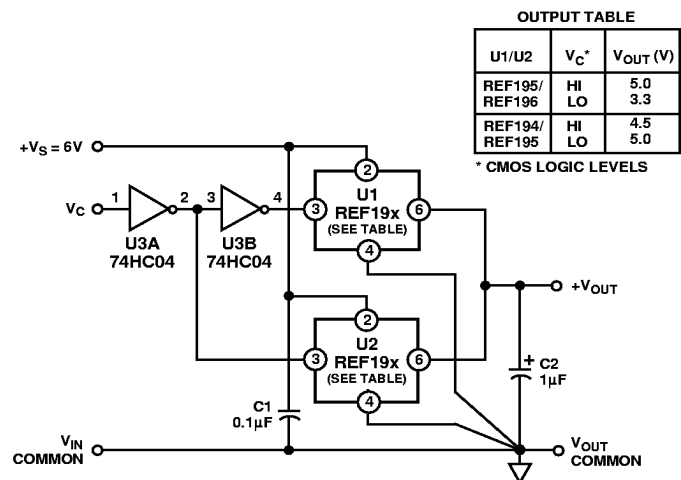
Figure 22. Switched Output Reference
