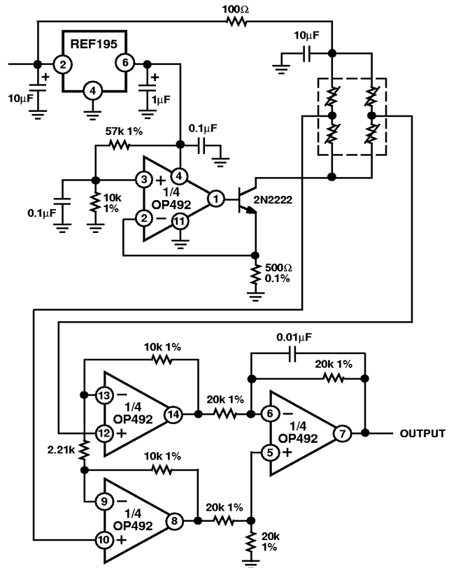
Figure 25. A Low Power, Strain Gage Circuit
