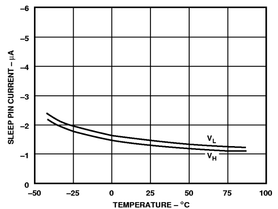
Figure 6. SLEEP Pin Current vs. Temperature
