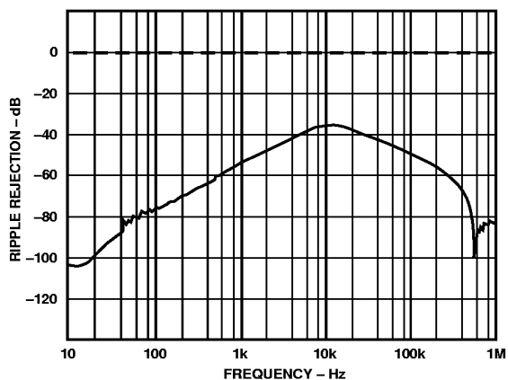
Figure 7a. Ripple Rejection vs. Frequency
