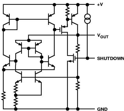
Figure 14. Simplified Schematic
