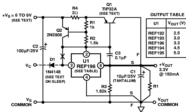
Figure 17. A Boosted 3.3 V Reference with Current Limiting
