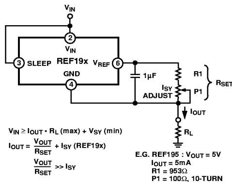
Figure 21. A Low Dropout, Precision Current Source
