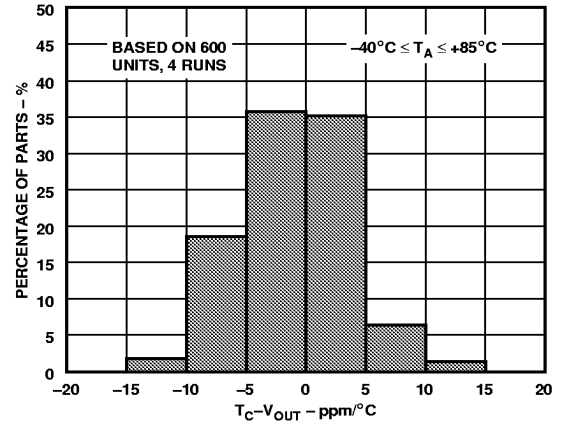
Figure 4. T_C - V_{OUT} Distribution
