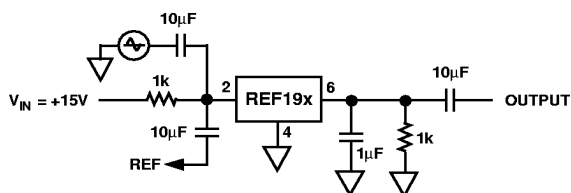
Figure 7b. Ripple Rejection vs. Frequency Measurement Circuit
