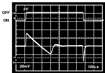
Figure 9a. Load Transient Response
