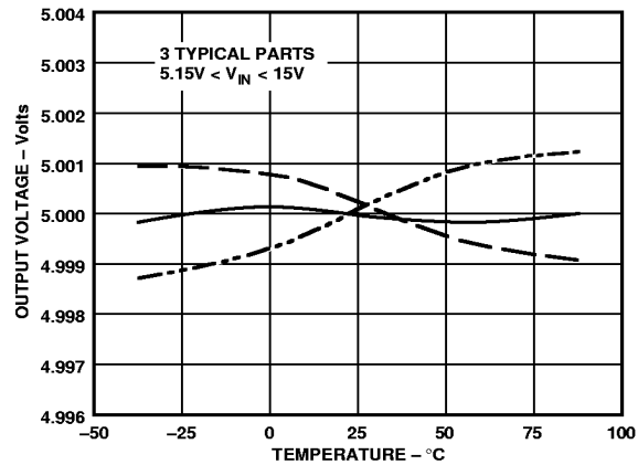
Figure 1. REF195 Output Voltage vs. Temperature
