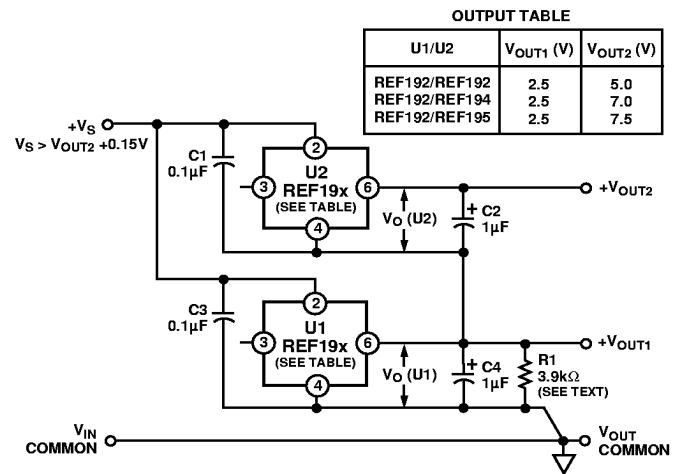
Figure 19. Stacking Voltage References with the REF19x
