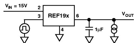
Figure 11b. Sleep Response Time Measurement Circuit
