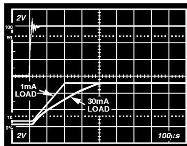
Figure 10a. Power ON Response Time
