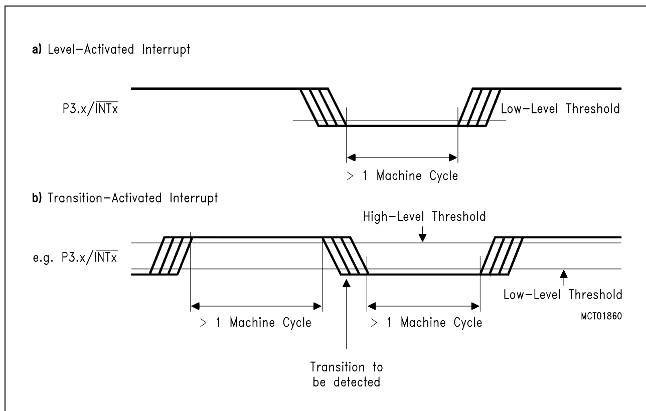
Figure 7-27 External Interrupt Detection
