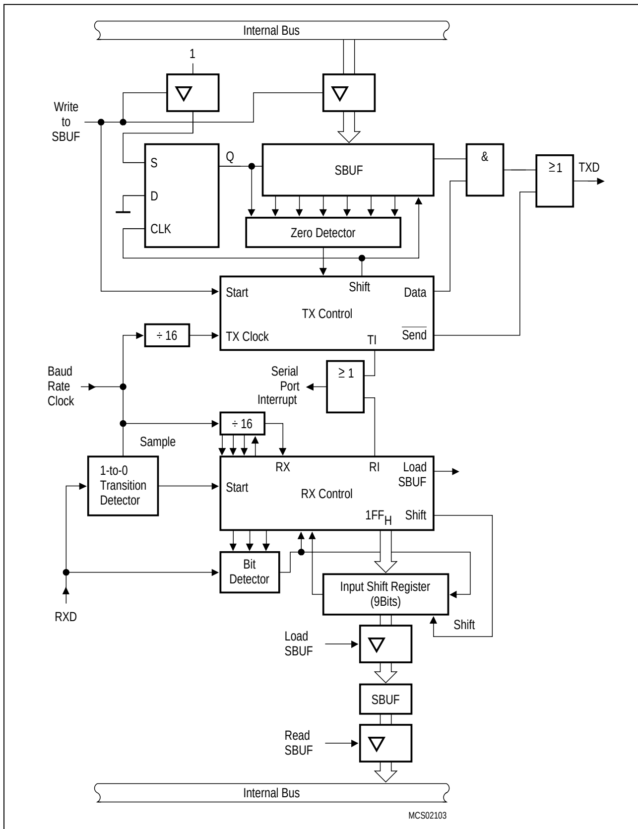
Figure 6-21 Serial Interface, Mode 1, Functional Diagram
