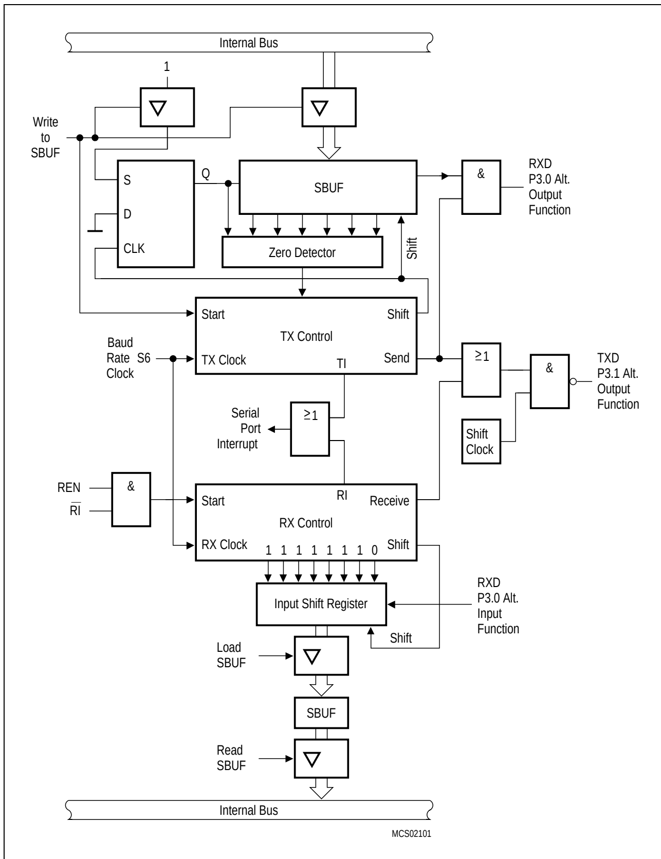
Figure 6-19 Serial Interface, Mode 0, Functional Diagram
