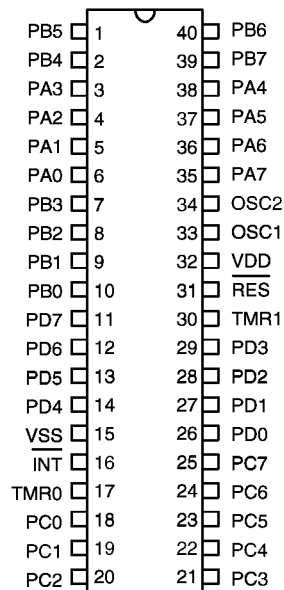
HT48R50 – 40 DIP-A-0
