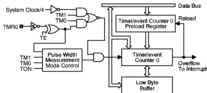
Timer/event counter 0
