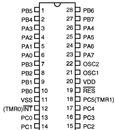
HT48R50 – 28 SKDIP-H-0
