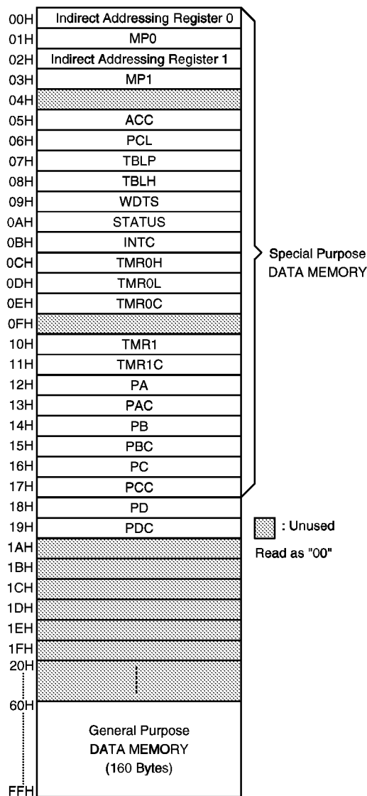
RAM mapping
