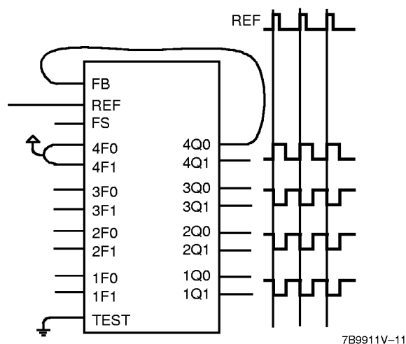
Figure 4. Inverted Output Connections
