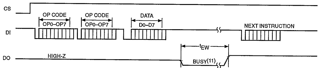
Figure 16. WRAL Timing (x8 Format)
