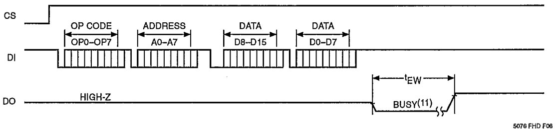
Figure 5. Program/Erase Timing (x16 Format)
