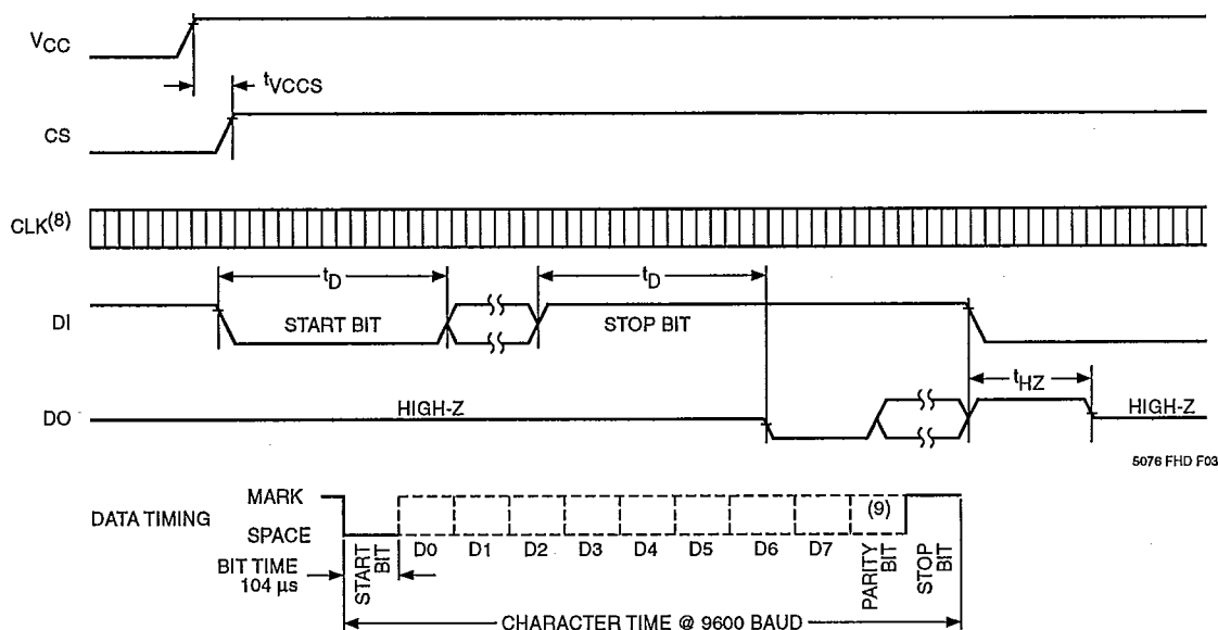
Figure 1. A.C. Timing
