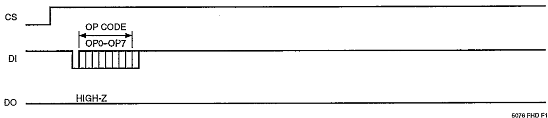
Figure 9. EWEN/EWDS Timing (x16 Format)
