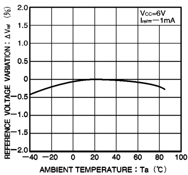
Fig.2 Reference voltage vs. ambient temperature
