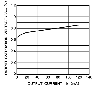
Fig.4 Output current vs. output saturation voltage
