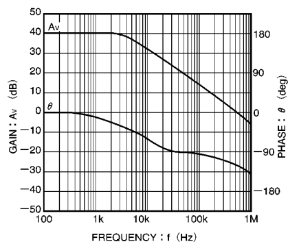
Fig.5 Error amplifier AC gain characteristic (40dB close)
