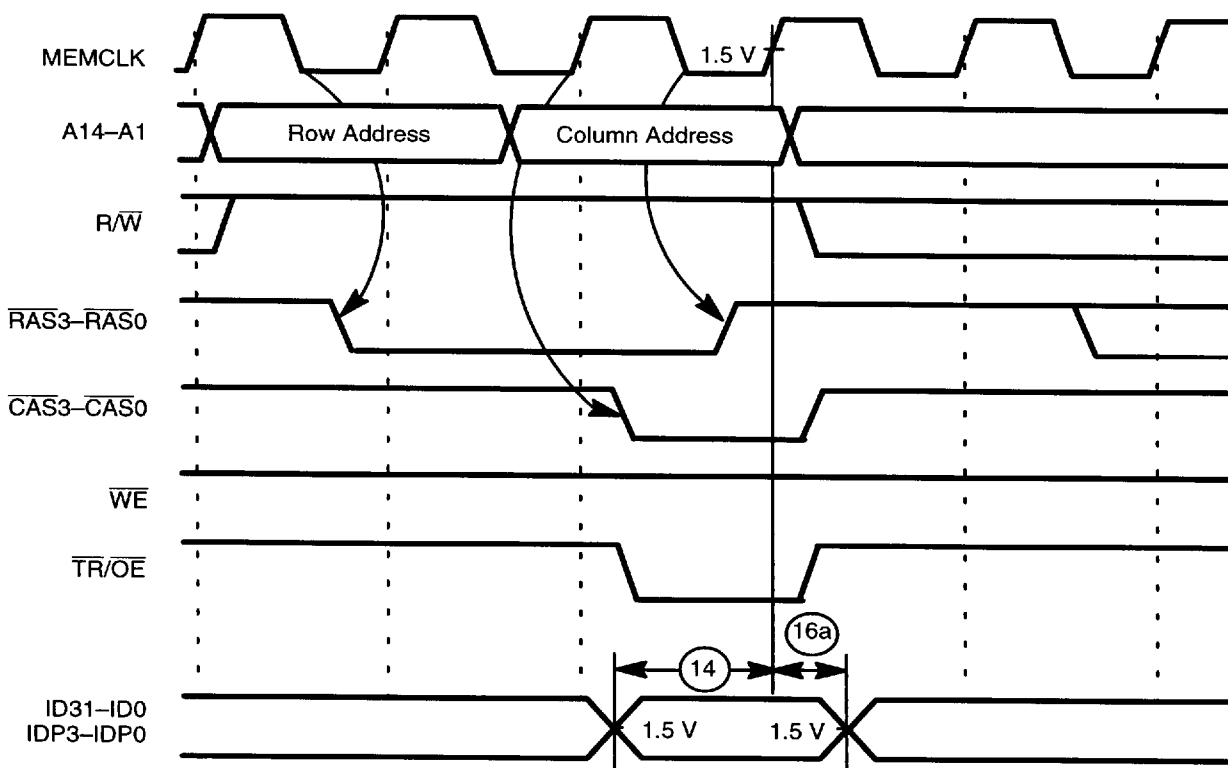
Figure 1. Simple 3/1 DRAM Read Cycle, Am29240 Microcontroller Series
