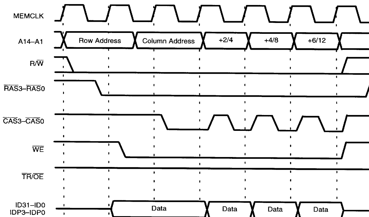
Figure 4. 3/1 DRAM Page-Mode Write, Am29240 Microcontroller Series
