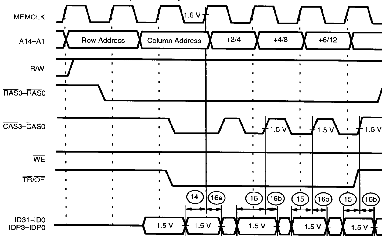
Figure 3. 3/1 DRAM Page-Mode Read, Am29240 Microcontroller Series
