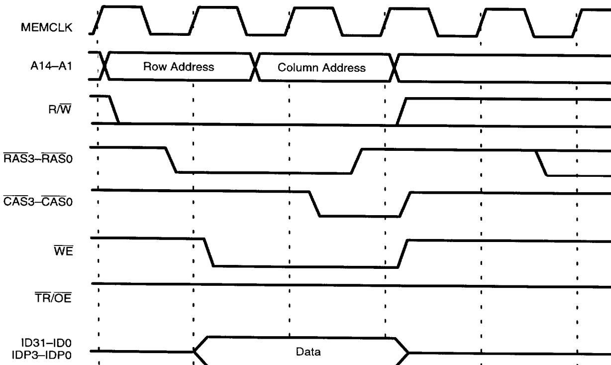
Figure 2. Simple 3/1 DRAM Write Cycle, Am29240 Microcontroller Series
