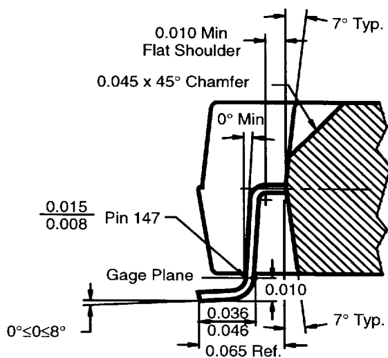
Detail X
