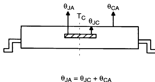
Figure 5. Thermal Resistance — °C/Watt
