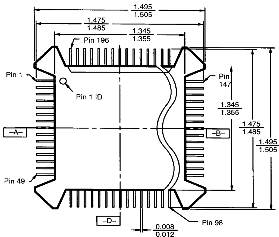
Top View
