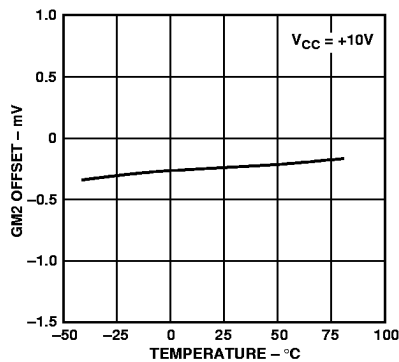
Figure 14. ADP3811 GM2 Offset vs. Temperature
