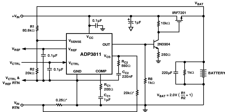
Figure 29. ADP3811 Controlling a Linear Battery Charger
