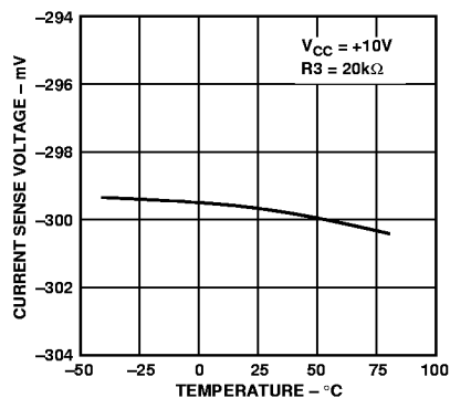
Figure 8. Full-Scale Current Sense Voltage vs. Temperature
