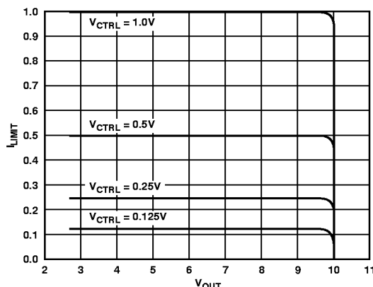
Figure 24. Charge Current vs. Battery Voltage at Four Settings for the Flyback Charger in Figure 23
