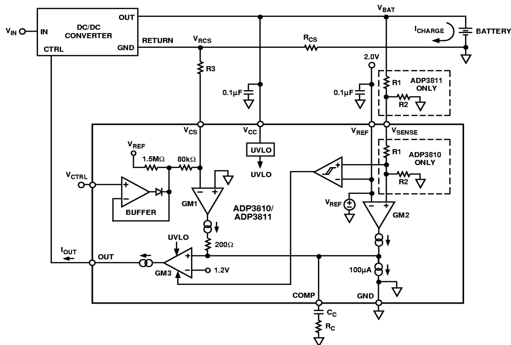
Figure 1. Simplified Battery Charger
