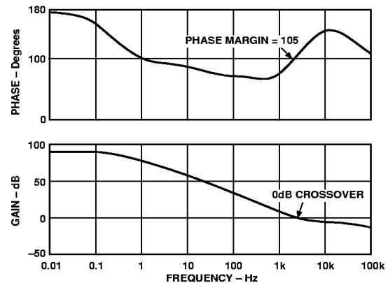
Figure 33. Current Loop Gain/Phase Plots
