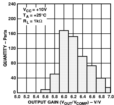
Figure 20. Output Gain ( V_{OUT}/V_{COMP} ) Distribution
