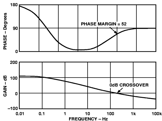
Figure 32. Voltage Loop Gain/Phase Plots
