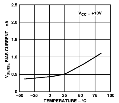
Figure 16. ADP3811 V_{SENSE} Bias Current vs. Temperature
