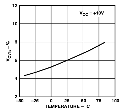
Figure 19. Overvoltage Comparator Threshold ( V_{OV\%} ) vs. Temperature
