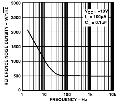
Figure 6. Reference Noise Density vs. Frequency
