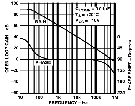
Figure 10. GM1 Open-Loop Gain and Phase vs. Frequency
