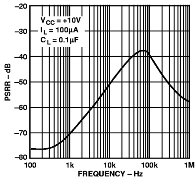
Figure 5. Reference PSRR vs. Frequency
