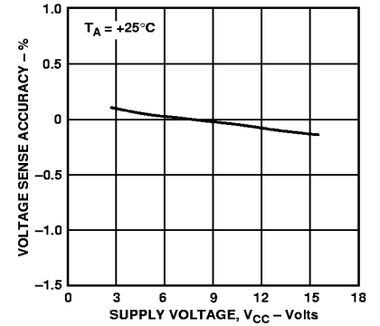
Figure 13. ADP3810 Voltage Sense Accuracy vs. V_{CC}
