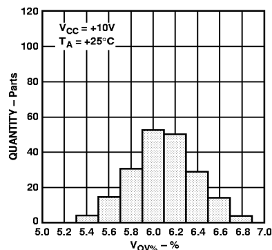
Figure 18. Overvoltage Comparator Distribution ( V_{OV\%} )
