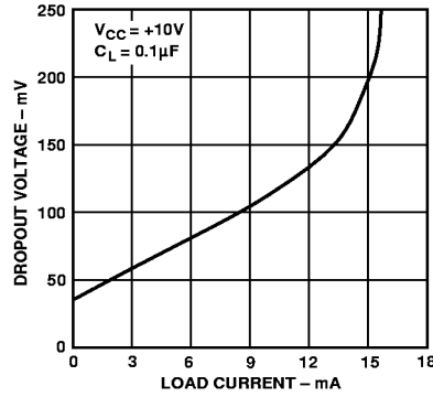
Figure 3. Reference Drop-Out Voltage ( V_{CC}-V_{REF} ) vs. Load Current
