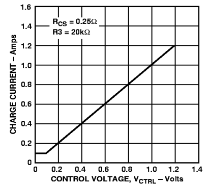
Figure 7. Charge Current vs. Control Voltage
