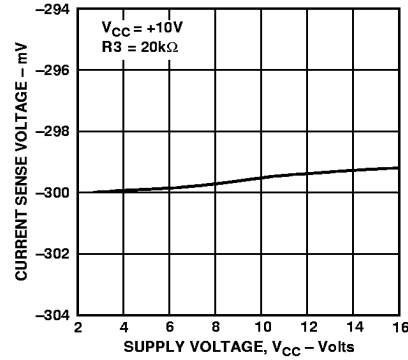
Figure 9. Full-Scale Current Sense Voltage vs. V_{CC}
