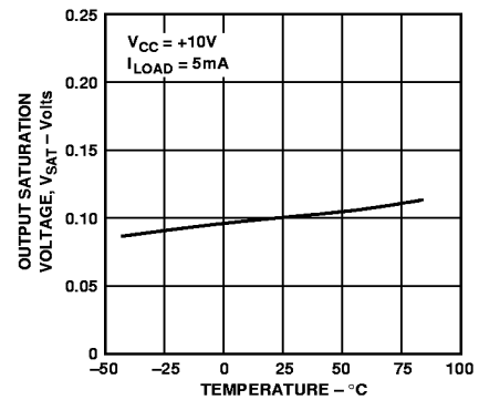
Figure 22. V_{SAT} vs. Temperature
