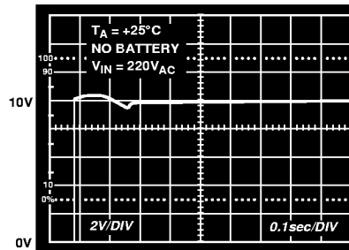
Figure 25. Flyback Charger Output Voltage Transient at Power Turn On, No Battery Attached
