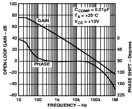
Figure 11. GM2 Open-Loop Gain and Phase vs. Frequency
