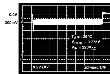
Figure 26. Charge Current Transient Response to Battery Connect/Disconnect
