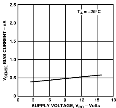
Figure 17. ADP3811 V_{SENSE} Bias Current vs. V_{CC}
