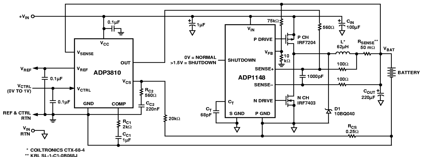
Figure 28. High Efficiency Buck Battery Charger
