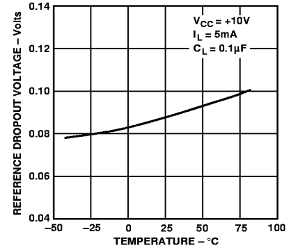
Figure 4. Reference Drop-Out Voltage vs. Temperature
