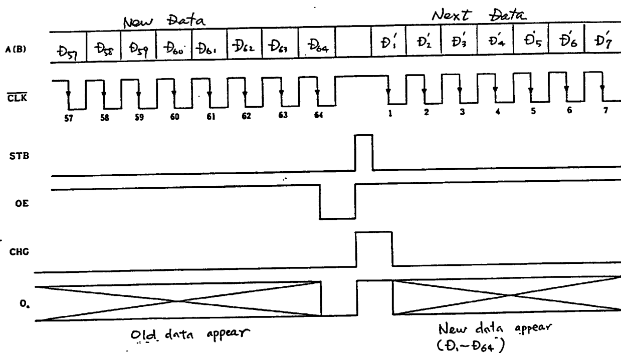
TIMING CHART (Using only one \mu PD16309)
