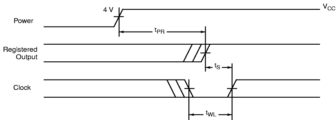
Figure 2. Power-Up Reset Waveform
