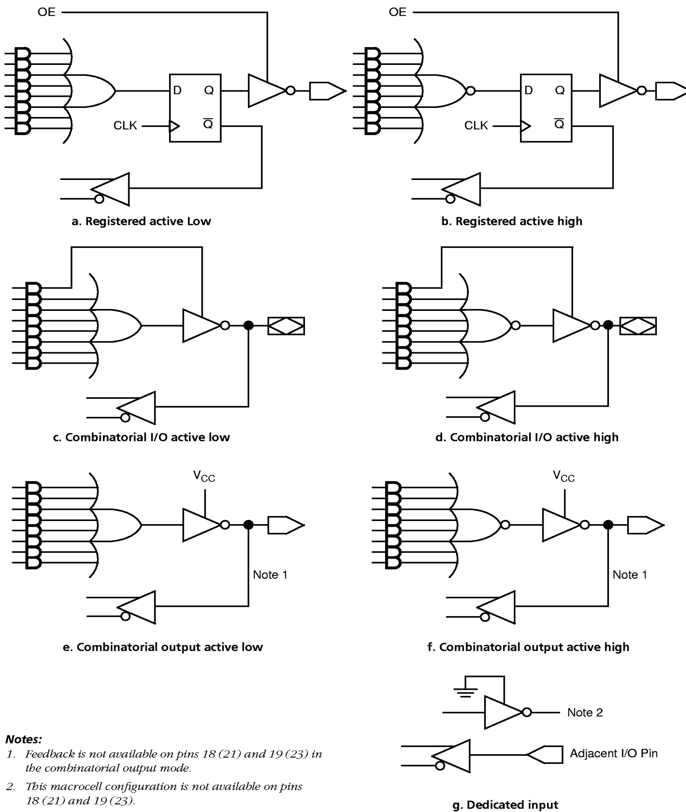
Figure 2. Macrocell Configurations
