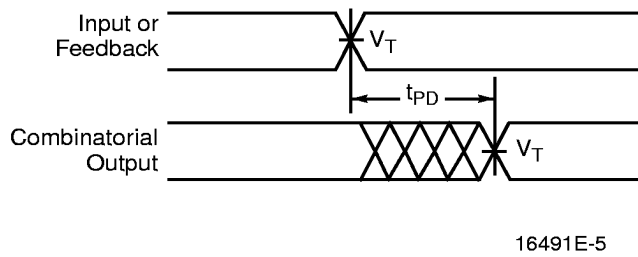
a. Combinational output
