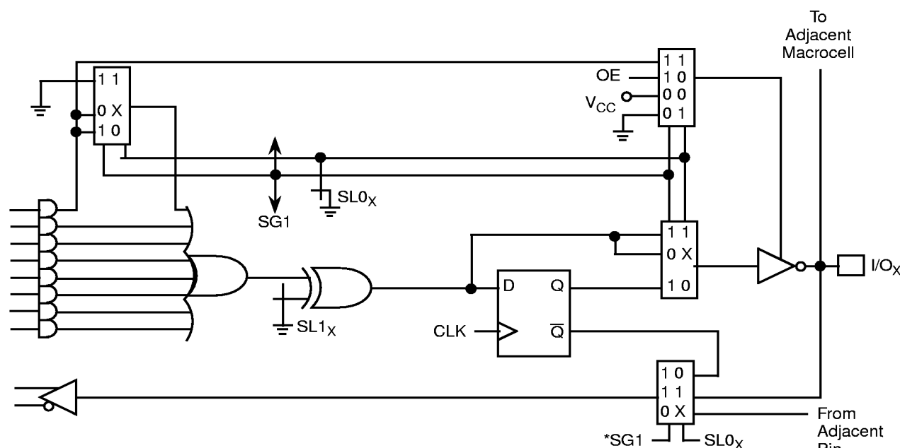
Figure 1. PALCE20V8 Macrocell
