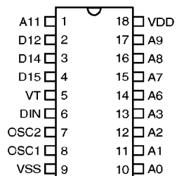
HT693 – 18 DIP
