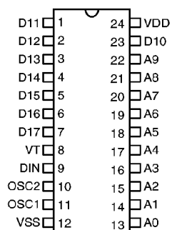
HT658 – 24 SOP/SDIP
