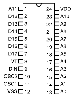
HT646L – 24 SOP/SDIP
