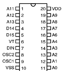
HT612 – 20 DIP/SOP
