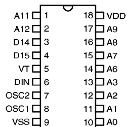
HT692 – 18 DIP
