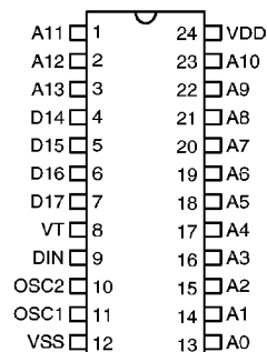
HT644L – 24 SOP/SDIP
