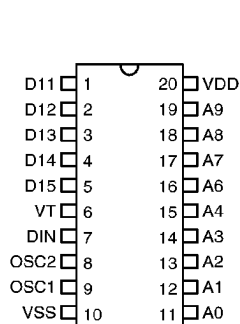
HT615 – 20 DIP/SOP
