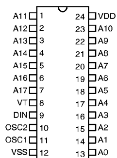
HT651 – 24 SOP/SDIP
