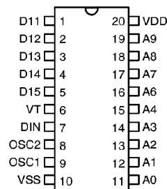
HT605L – 20 DIP/SOP
