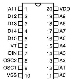
HT604L – 20 DIP/SOP
