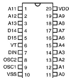
HT602L – 20 DIP/SOP
