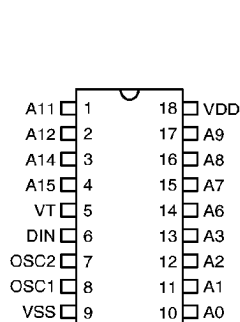
HT691 – 18 DIP
