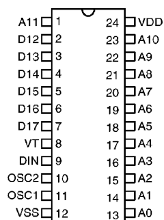
HT656 – 24 SOP/SDIP
