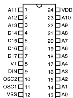
HT654 – 24 SOP/SDIP
