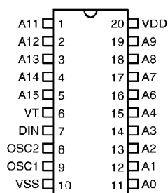
HT611 – 20 DIP/SOP
