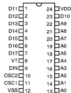
HT648L – 24 SOP/SDIP
