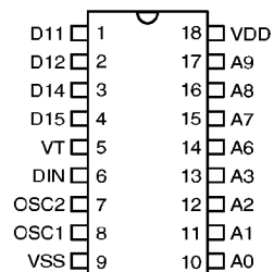
HT694 – 18 DIP
