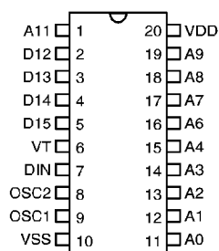
HT614 – 20 DIP/SOP
