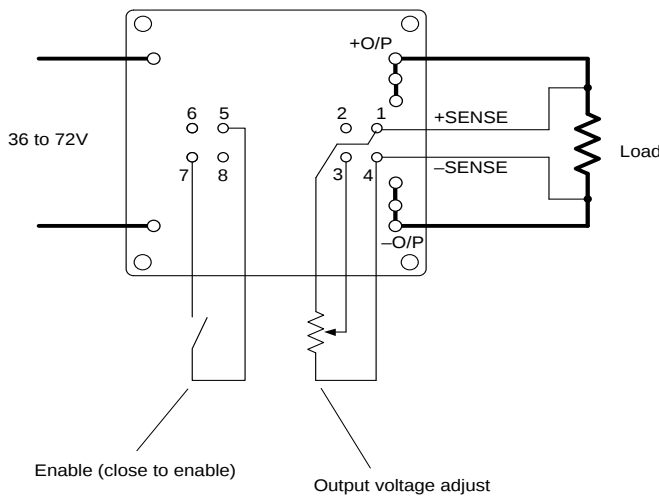
Connection example
