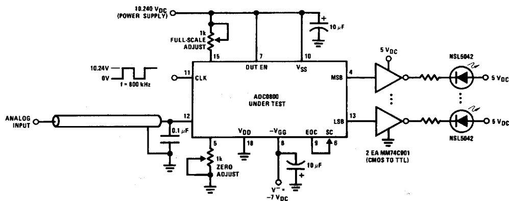
FIGURE 4. Complete Basic Tester Circuit
