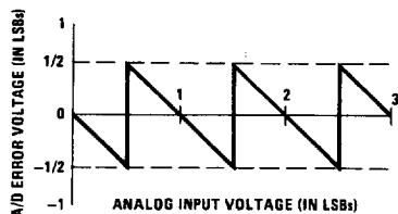
FIGURE 5. Error Plot of a Perfect A/D Showing Effects of Quantization Error
