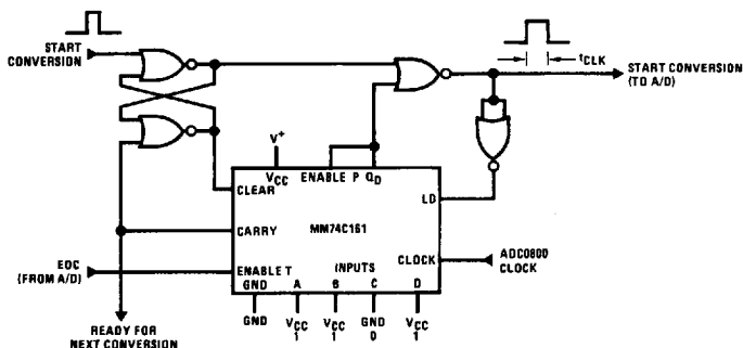
FIGURE 2. A/D Control Logic
