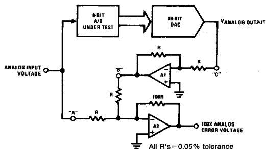
FIGURE 6. A/D Tester with Analog Error Output
