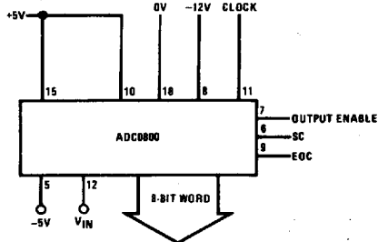
General Connection
