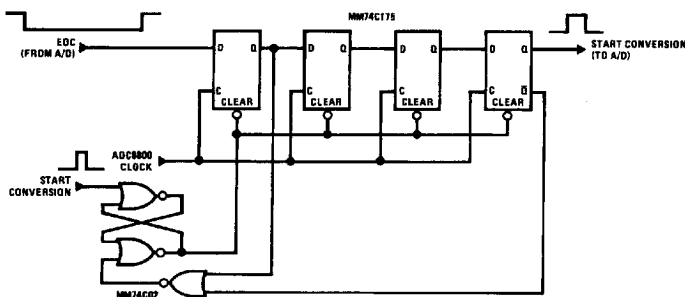
FIGURE 1. Delaying an Asynchronous Start Pulse
