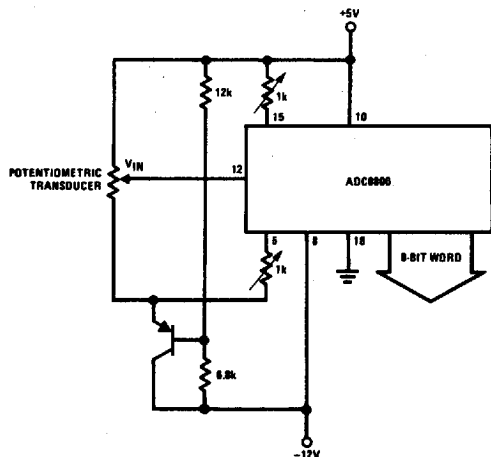
Ratiometric Input Signal with Tracking Reference
