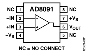
Figure 1. SOIC-8 (R-8)
