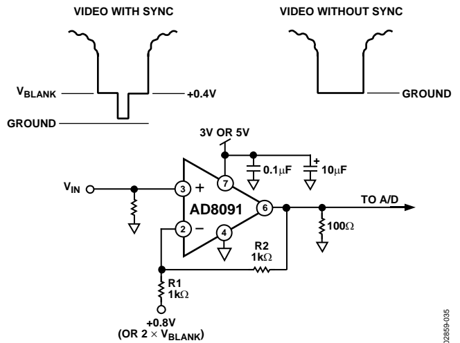
Figure 35. Sync Stripper
