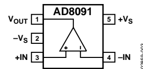
Figure 2. SOT23-5 (RT-5)
