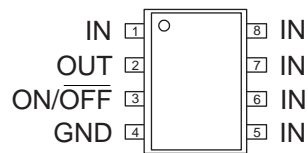
SC70JW-8 (Top View)
