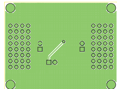
Figure 3: Evaluation Board Solder Side Layout.
