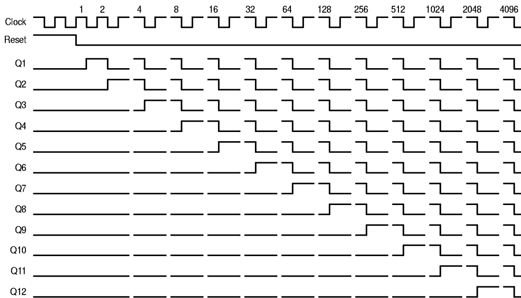
Figure 6. Timing Diagram
