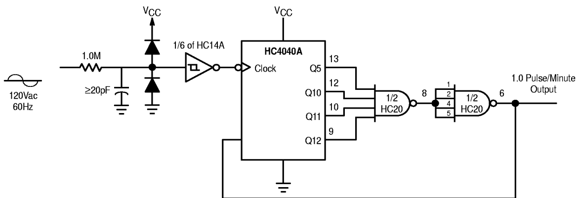
Figure 7. Time-Base Generator
