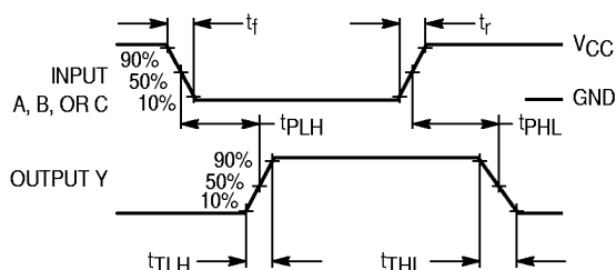
Figure 1. Switching Waveforms
