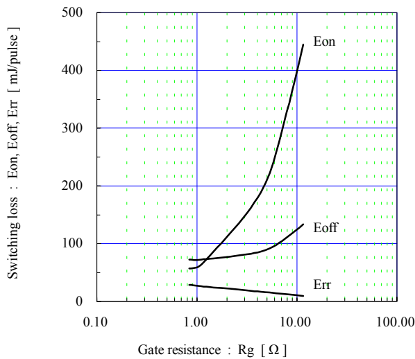
Switching loss vs. Gate resistance (typ.) V_{cc}=600V , I_c=600A , V_{GE}=\pm 15V , T_j=125^\circ C
