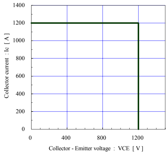
Reverse bias safe operating area (max.) +V_{GE}=15V , -V_{GE} \leq 15V , R_g \geq 1.1\Omega , T_j \leq 125^\circ C
