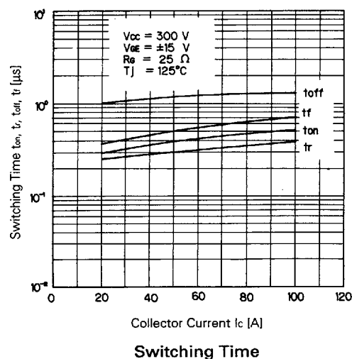
Switching Time
