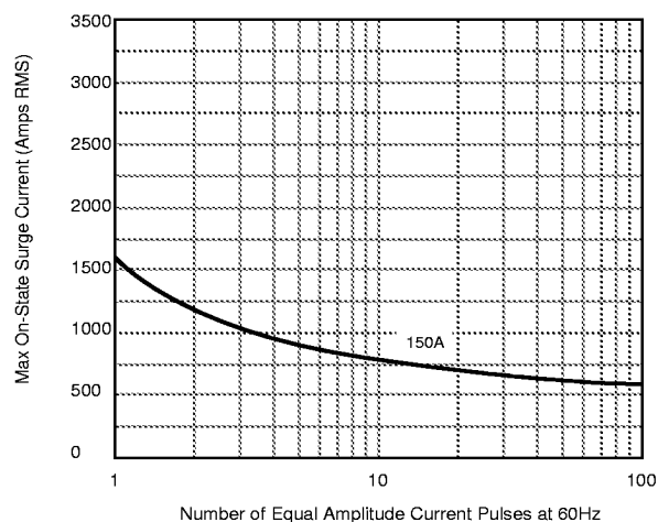
FIGURE 1 Max Non-Repetitive Surge Current
