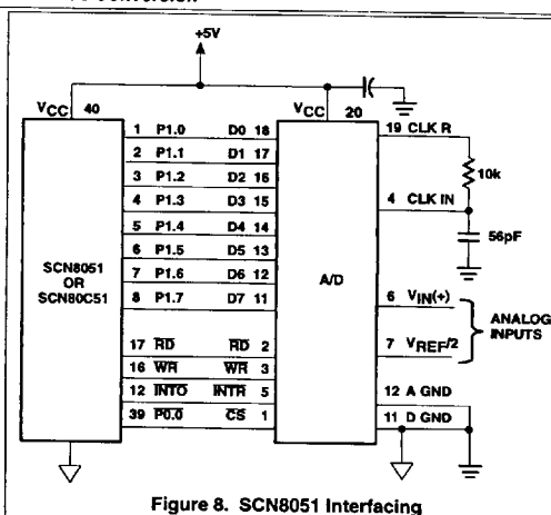
Figure 8. SCN8051 Interfacing
