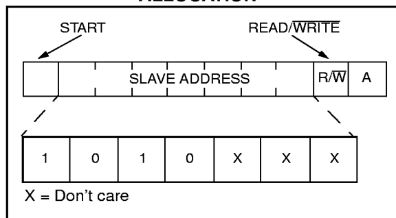
FIGURE 4-1: CONTROL BYTE ALLOCATION
