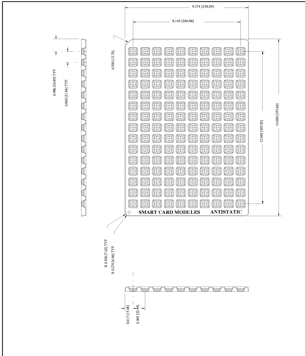
FIGURE 8-1: TRAY DIMENSIONS
