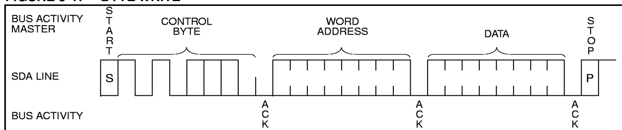
FIGURE 5-1: BYTE WRITE
