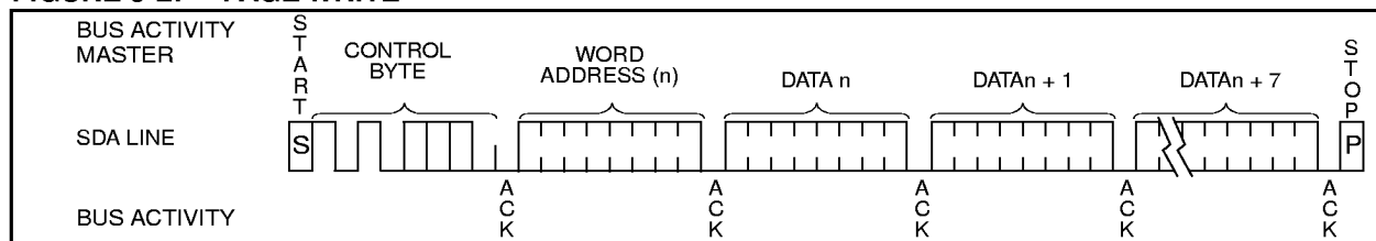
FIGURE 5-2: PAGE WRITE
