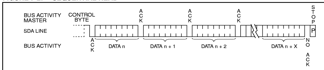
FIGURE 7-2: SEQUENTIAL READ
