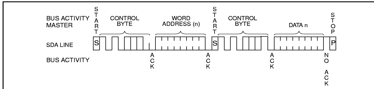
FIGURE 7-1: RANDOM READ
